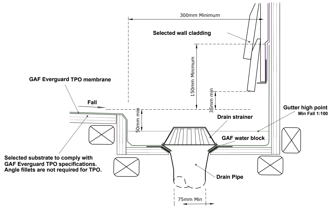
Drain / Dropper
