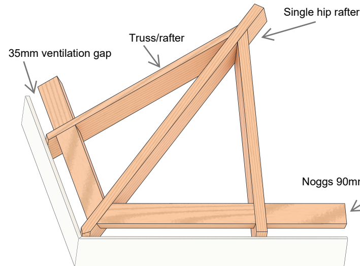
Valley detail
