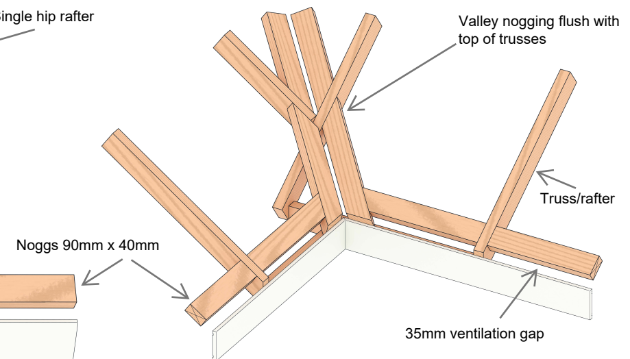
Valley detail
